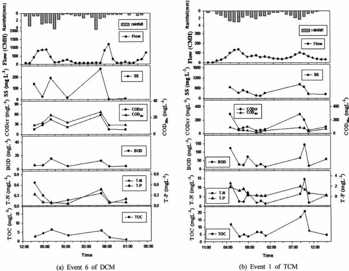
Fig. 2. Pollutant Concentration by DCM, TCM.
